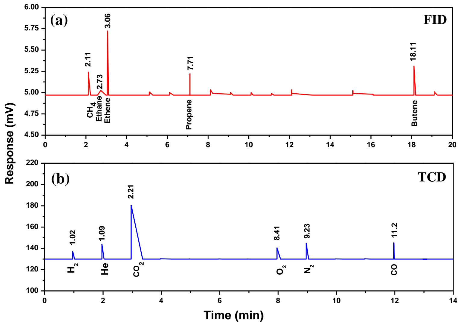
Fig. 10. The gas chromatography analysis of gaseous products in case of molten carbonate electrolysis by (a) FID detector (b) TCD detector.
