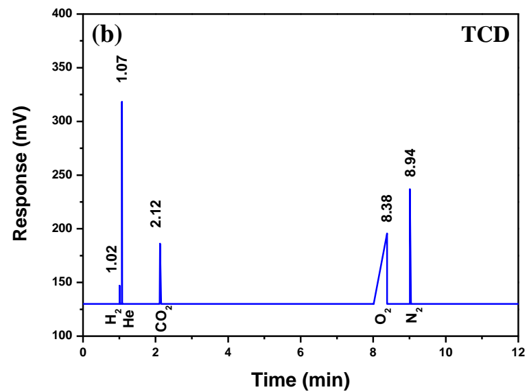
Fig. 5. The gas chromatography analysis of gaseous products in case of molten chloride electrolysis at 375 °C and 2 V by (a) FID detector (b) TCD detector.
