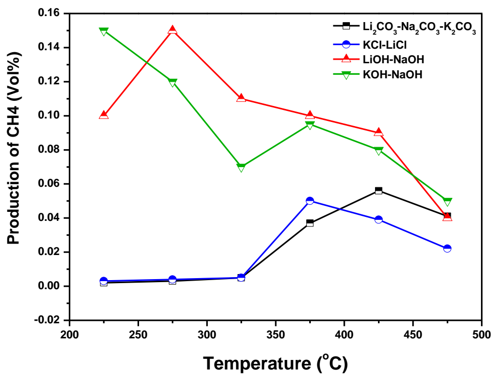
Fig. 11. The selection of optimum temperatures for all electrolytes on the basis of \text{CH}_4 production.
