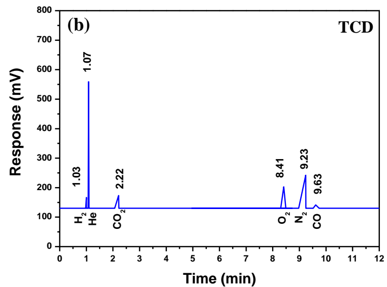
Fig. 7. The gas chromatography analysis of gaseous products in case of molten hydroxide (LiOH-NaOH) electrolysis by (a) FID detector (b) TCD detector.
