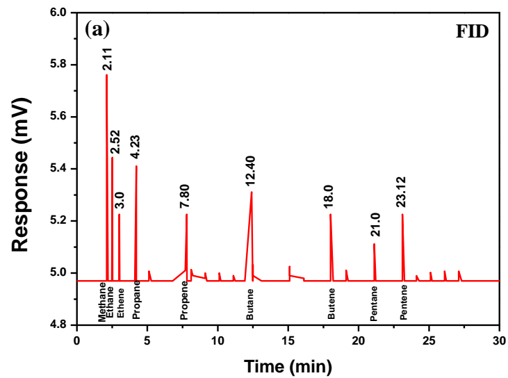
Fig. 2. The gas chromatography analysis of calibration gas standards as reference for the comparison with other electrolysis gaseous products by (a) FID detector (b) TCD detector.
